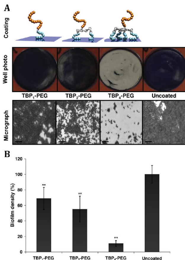
Figure 9. (Top) Illustration of the bacteriophobic coatings possessing one or more bottom TBPs (blue), a peptide linker (silver), and a top PEG domain (gold). Schematic of three bacteriophobic coatings under investigation where one (left), two (middle), or four (right) titanium-binding peptides (TBPs) are covalently attached to a polyethylene glycol (PEG). Digital photographs and (bottom) phase-contrast micrographs (Magnification = 630 \times ) of coated and uncoated Ti wells following a 5 h exposure to S. aureus cultures (starting inoculum of \sim 5 \times 10^7 CFUs/mL). Bacteria were stained with 0.1% crystal violet to aid visualization. Scale bars = 20 \mu m. (Bottom) Quantification of biofilm formation on coated and uncoated Ti surfaces following a 5 h exposure to S. aureus (starting inoculum of \sim 5 \times 10^7 CFUs/mL) cultures. ( N = 3 , **P < 0.01 ). Reprinted with permission from ref 88. Copyright 2010 Elsevier Ltd.
